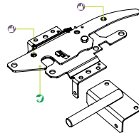
5" x 5" Standard Post Latch Vinyl SS
