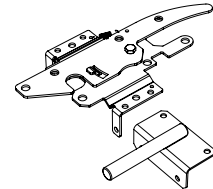
5" x 5" Standard Post Latch Vinyl SS
